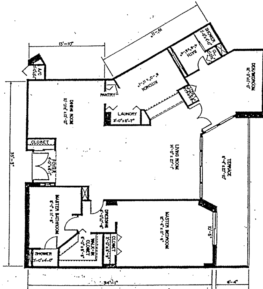
MEZZANINE, 2ND FLOOR & TYPICAL FLOOR APARTMENT A FLOOR PLAN THE HAMPTONS WEST A CONDOMINIUM REV. 10/24/11 ISSUED OCTOBER 10, 2011
